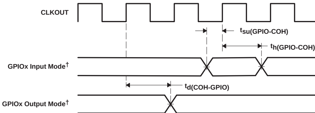
Figure 41. GPIOx ^\dagger Timings
