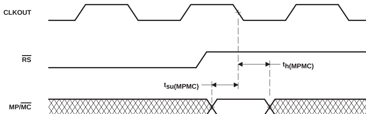
Figure 27. \text{MP}/\overline{\text{MC}} Timing
