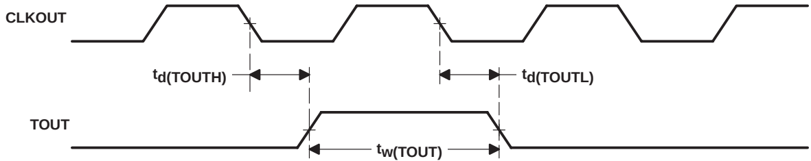
Figure 30. TOUT Timing
